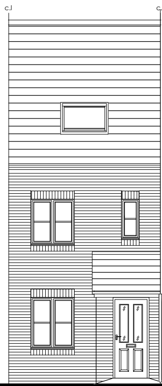
Front Elevation
